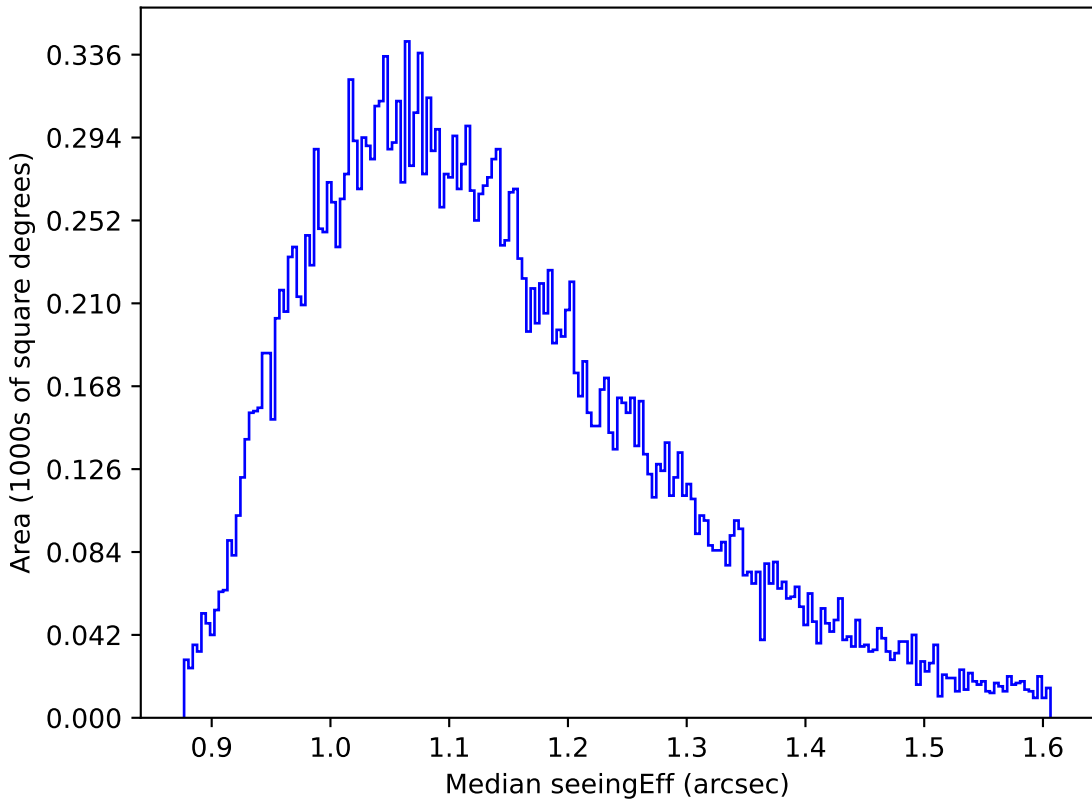
too_elab_r8_d3_giz_v3.4_10yrs All sky g band: Median seeingEff
