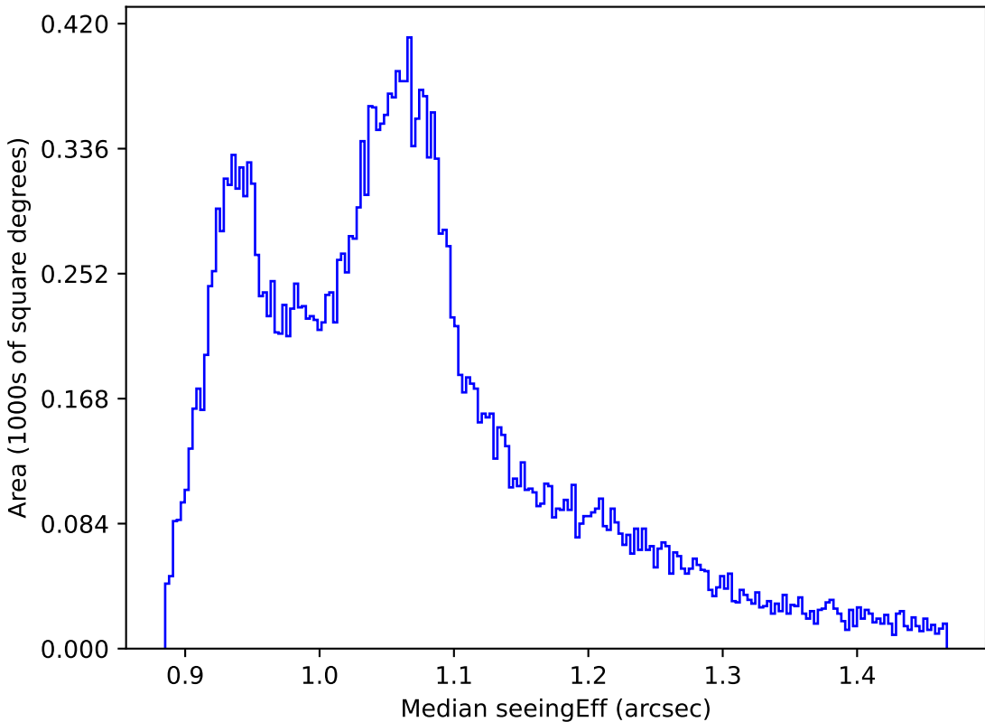
too_elab_r8_d3_giz_v3.4_10yrs All sky all bands: Median seeingEff
