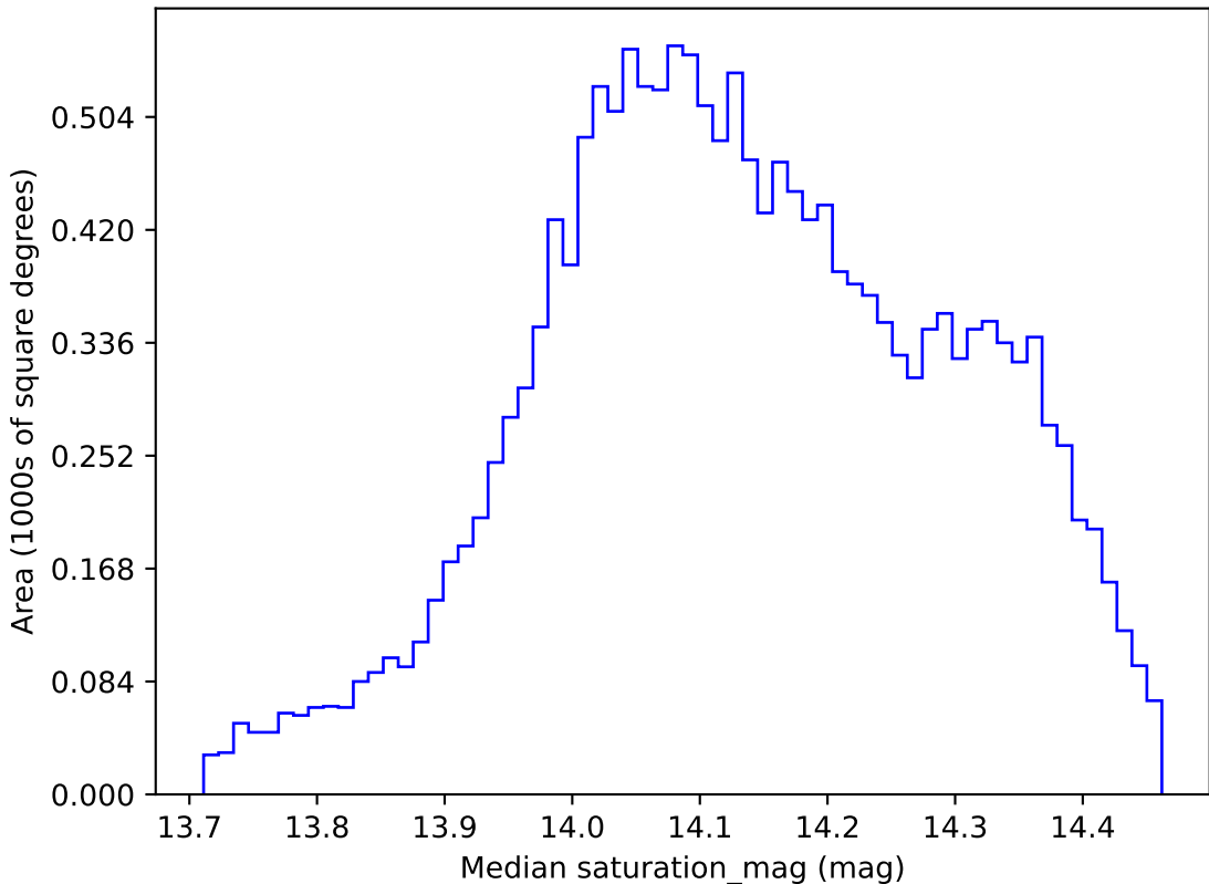
too_elab_r8_d3_giz_v3.4_10yrs WFD z band: Median saturation_mag
