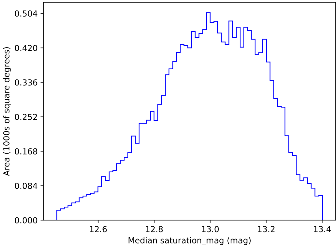
too_elab_r8_d3_giz_v3.4_10yrs WFD u band: Median saturation_mag
