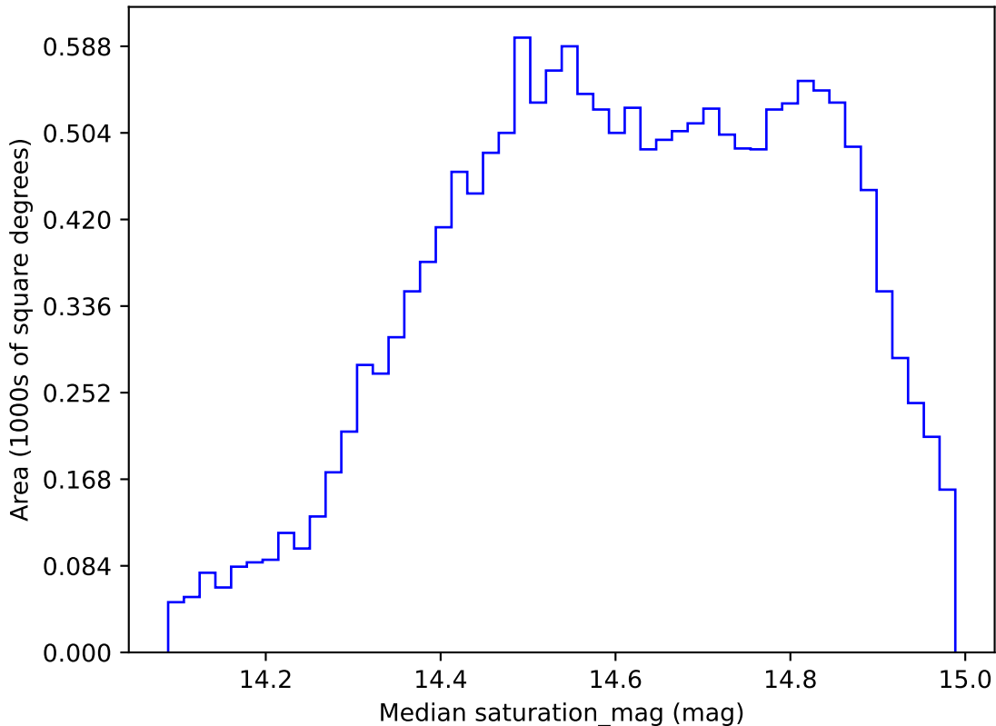
too_elab_r8_d3_giz_v3.4_10yrs WFD r band: Median saturation_mag
