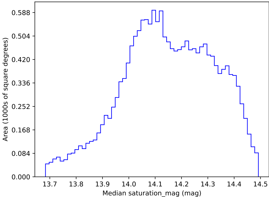
too_elab_r8_d3_giz_v3.4_10yrs WFD all bands: Median saturation_mag
