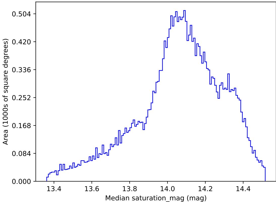
too_elab_r8_d3_giz_v3.4_10yrs All sky z band: Median saturation_mag
