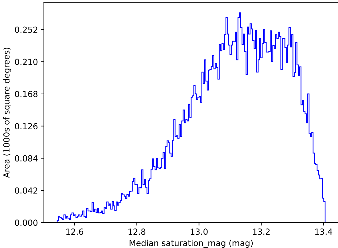
too_elab_r8_d3_giz_v3.4_10yrs All sky y band: Median saturation_mag
