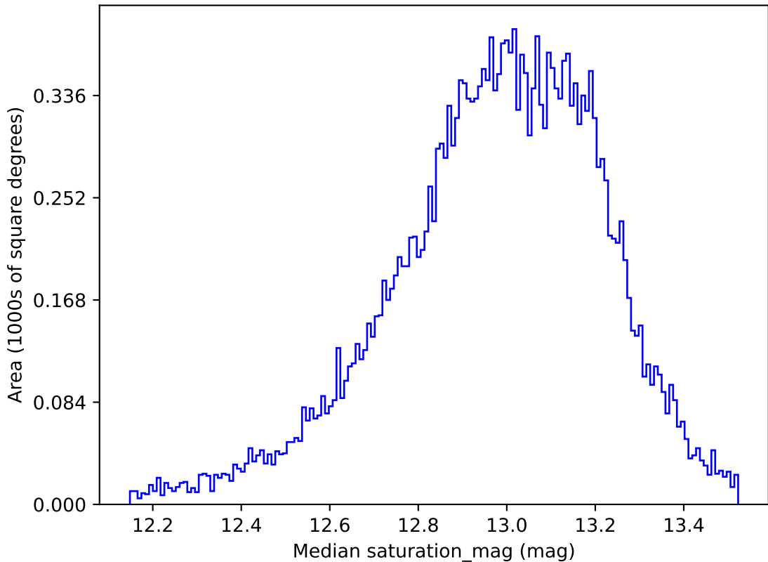
too_elab_r8_d3_giz_v3.4_10yrs All sky u band: Median saturation_mag
