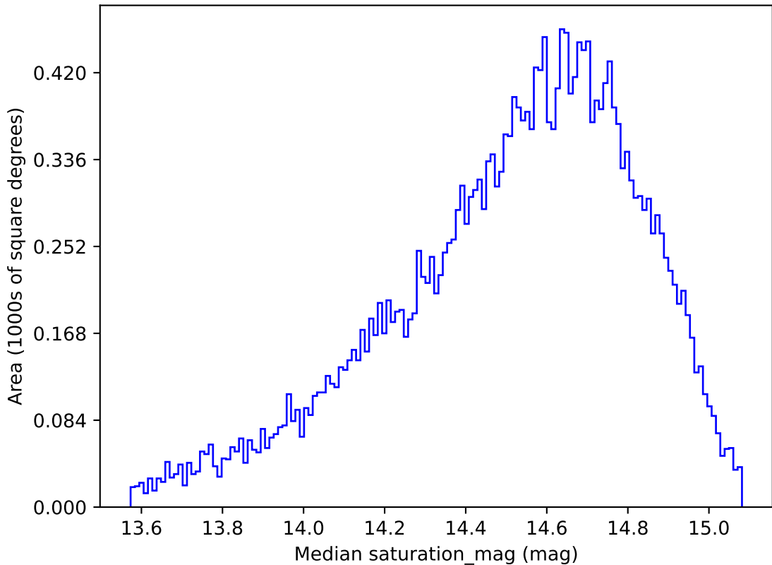
too_elab_r8_d3_giz_v3.4_10yrs All sky g band: Median saturation_mag
