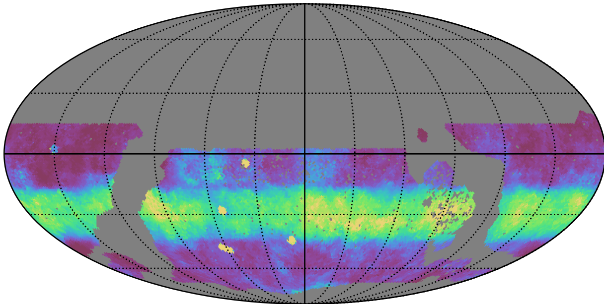
too_elab_r8_d3_giz_v3.4_10yrs WFD z band: Median normairmass
