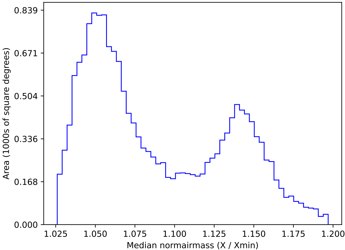
too_elab_r8_d3_giz_v3.4_10yrs WFD y band: Median normairmass
