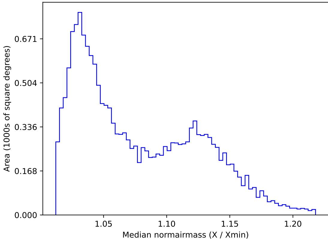
too_elab_r8_d3_giz_v3.4_10yrs WFD u band: Median normairmass
