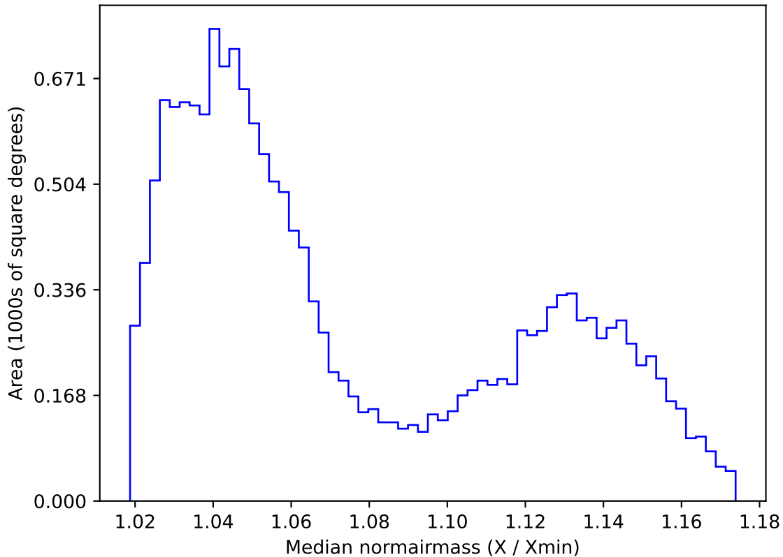
too_elab_r8_d3_giz_v3.4_10yrs WFD i band: Median normairmass
