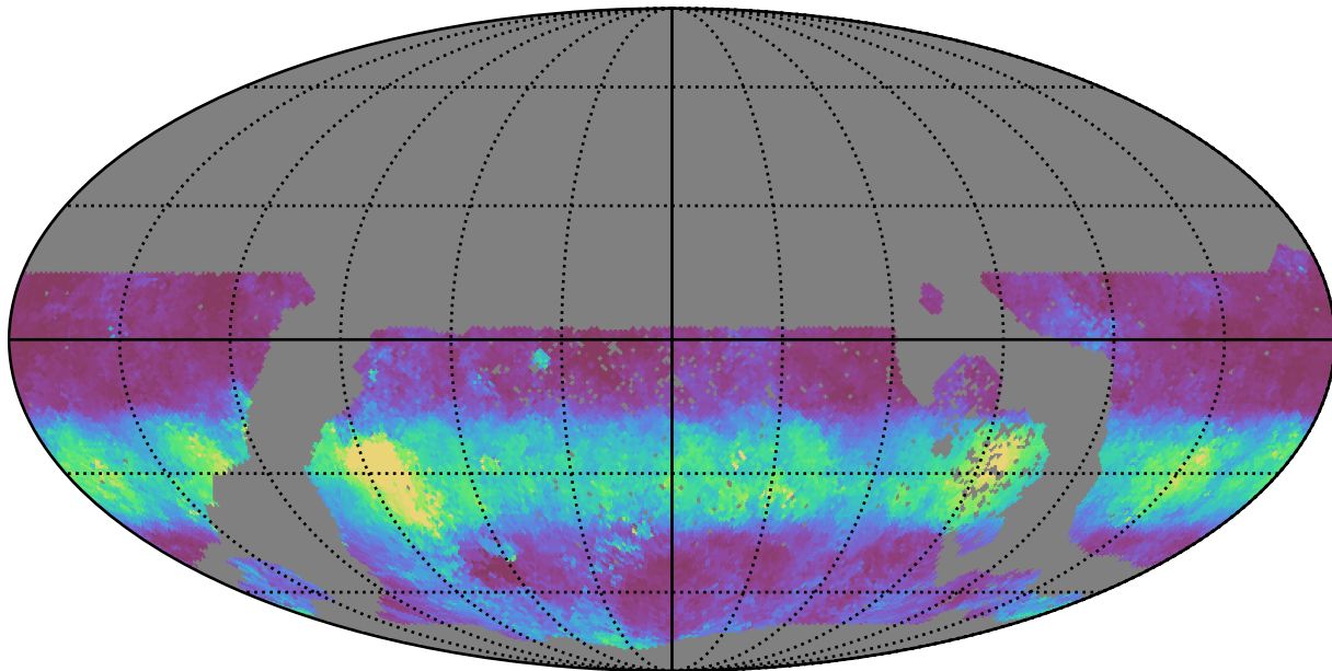
too_elab_r8_d3_giz_v3.4_10yrs WFD g band: Median normairmass
