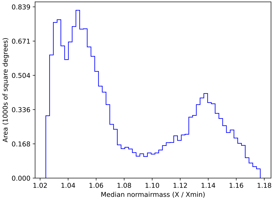
too_elab_r8_d3_giz_v3.4_10yrs WFD all bands: Median normairmass
