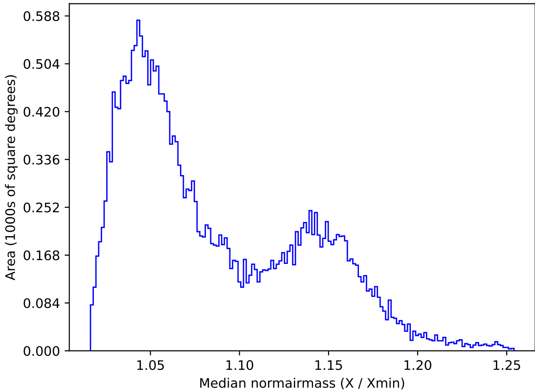
too_elab_r8_d3_giz_v3.4_10yrs All sky z band: Median normairmass
