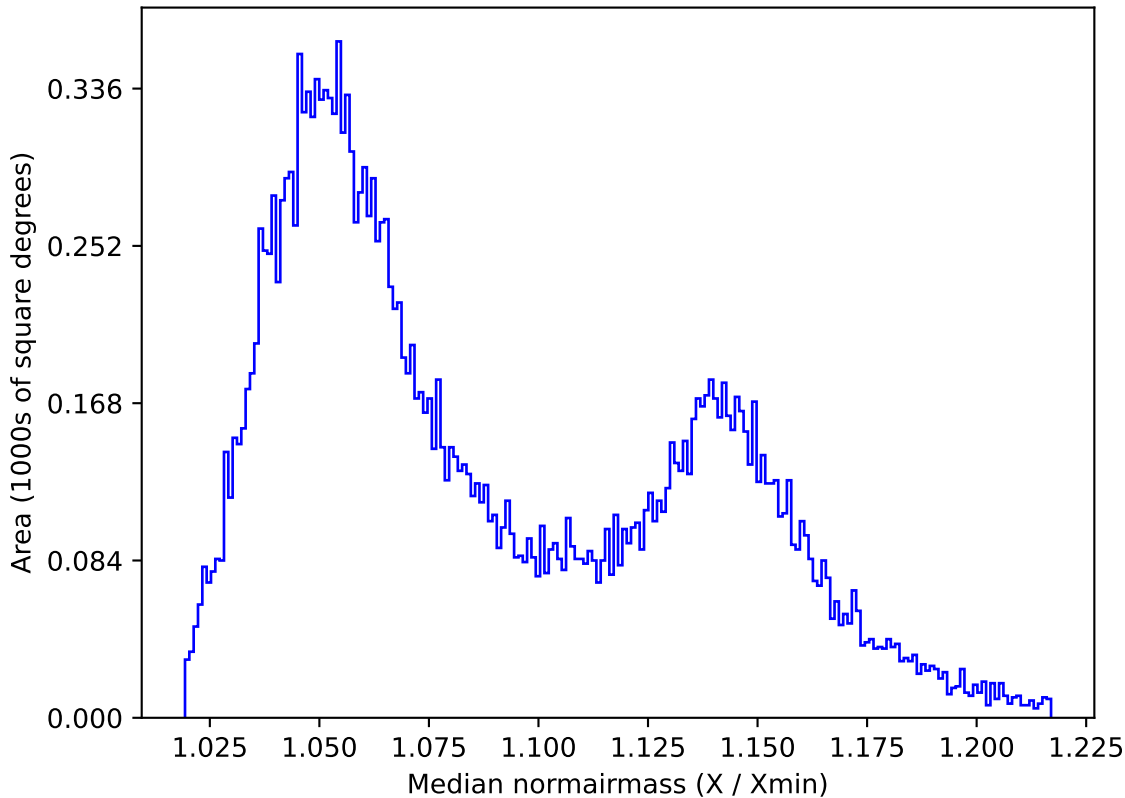
too_elab_r8_d3_giz_v3.4_10yrs All sky y band: Median normairmass
