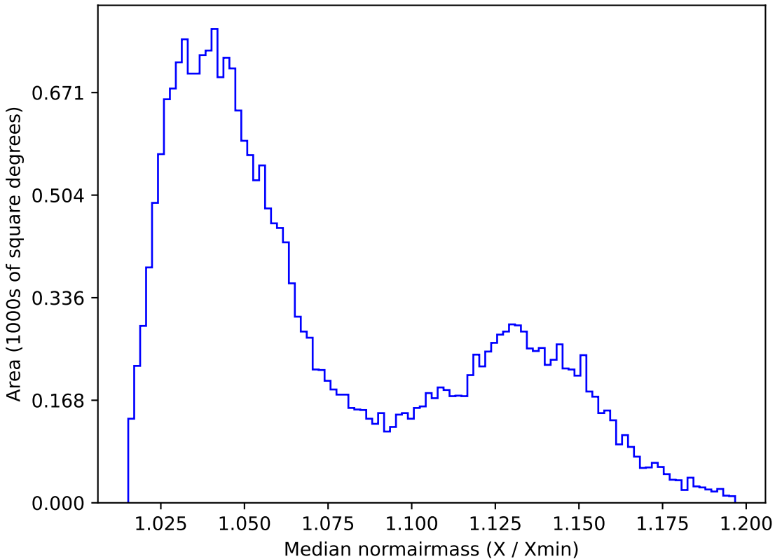
too_elab_r8_d3_giz_v3.4_10yrs All sky i band: Median normairmass
