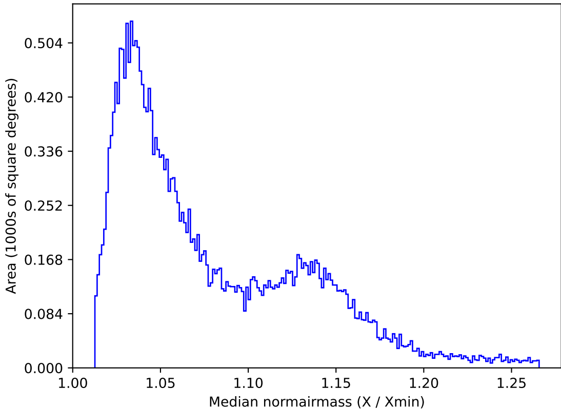
too_elab_r8_d3_giz_v3.4_10yrs All sky g band: Median normairmass
