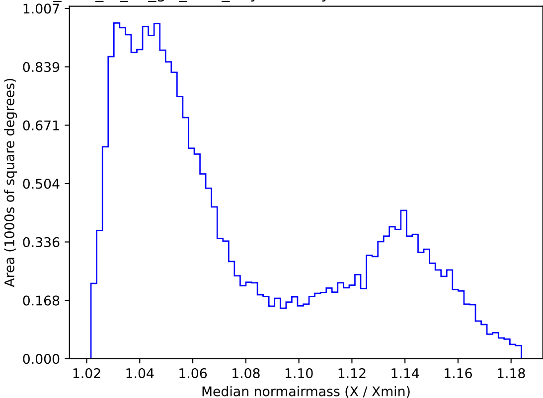
too_elab_r8_d3_giz_v3.4_10yrs All sky all bands: Median normairmass
