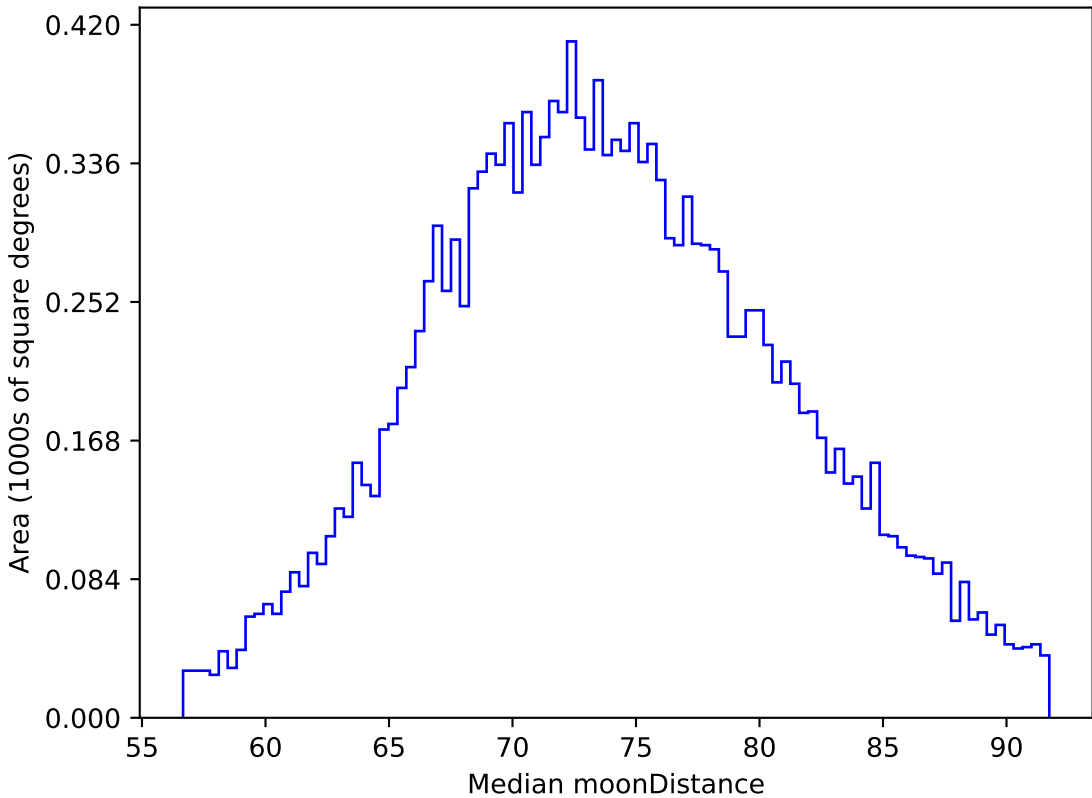
too_elab_r8_d3_giz_v3.4_10yrs WFD z band: Median moonDistance
