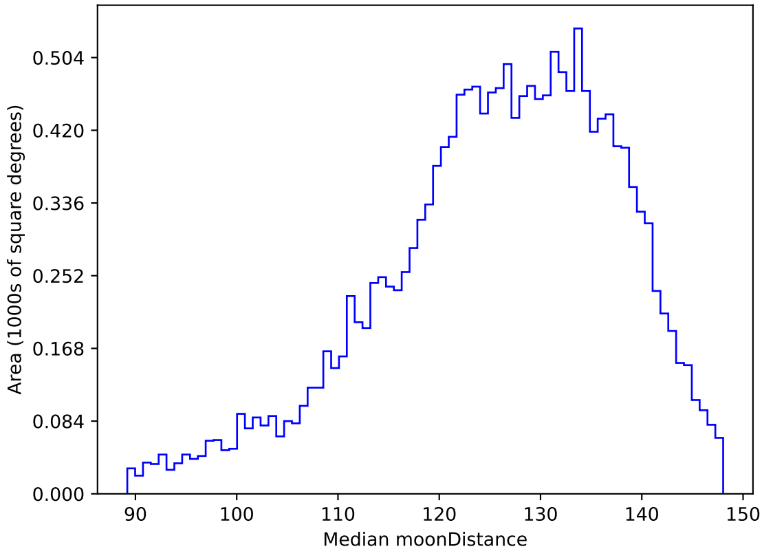
too_elab_r8_d3_giz_v3.4_10yrs WFD u band: Median moonDistance
