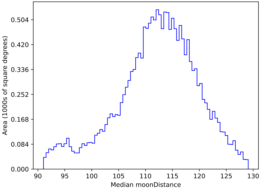
too_elab_r8_d3_giz_v3.4_10yrs WFD r band: Median moonDistance
