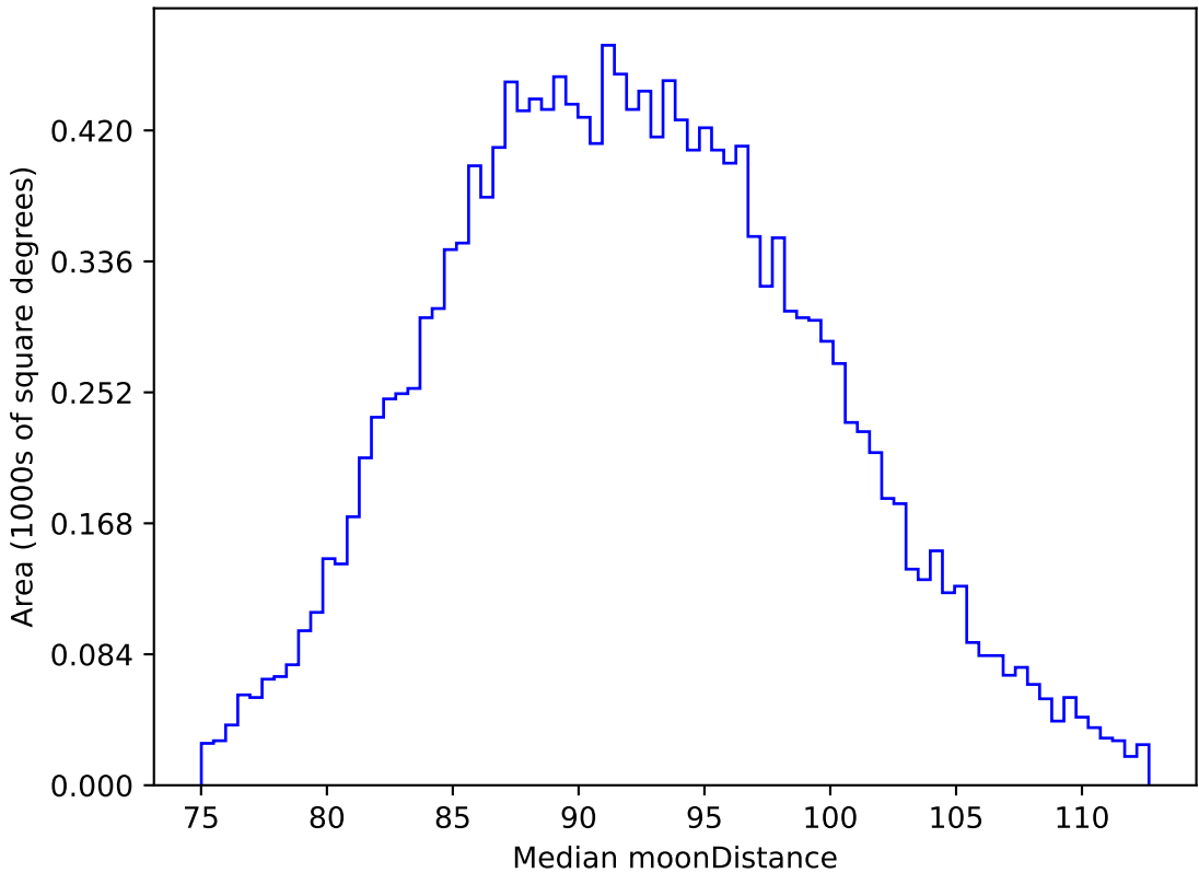
too_elab_r8_d3_giz_v3.4_10yrs WFD i band: Median moonDistance
