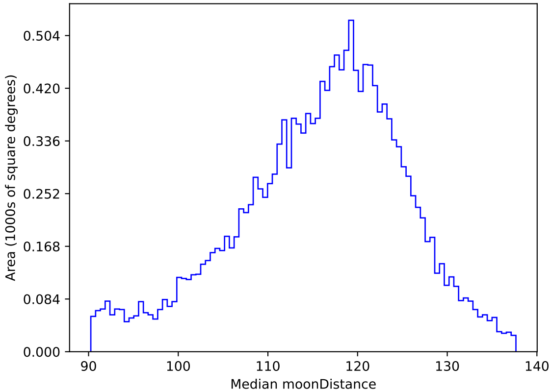
too_elab_r8_d3_giz_v3.4_10yrs WFD g band: Median moonDistance
