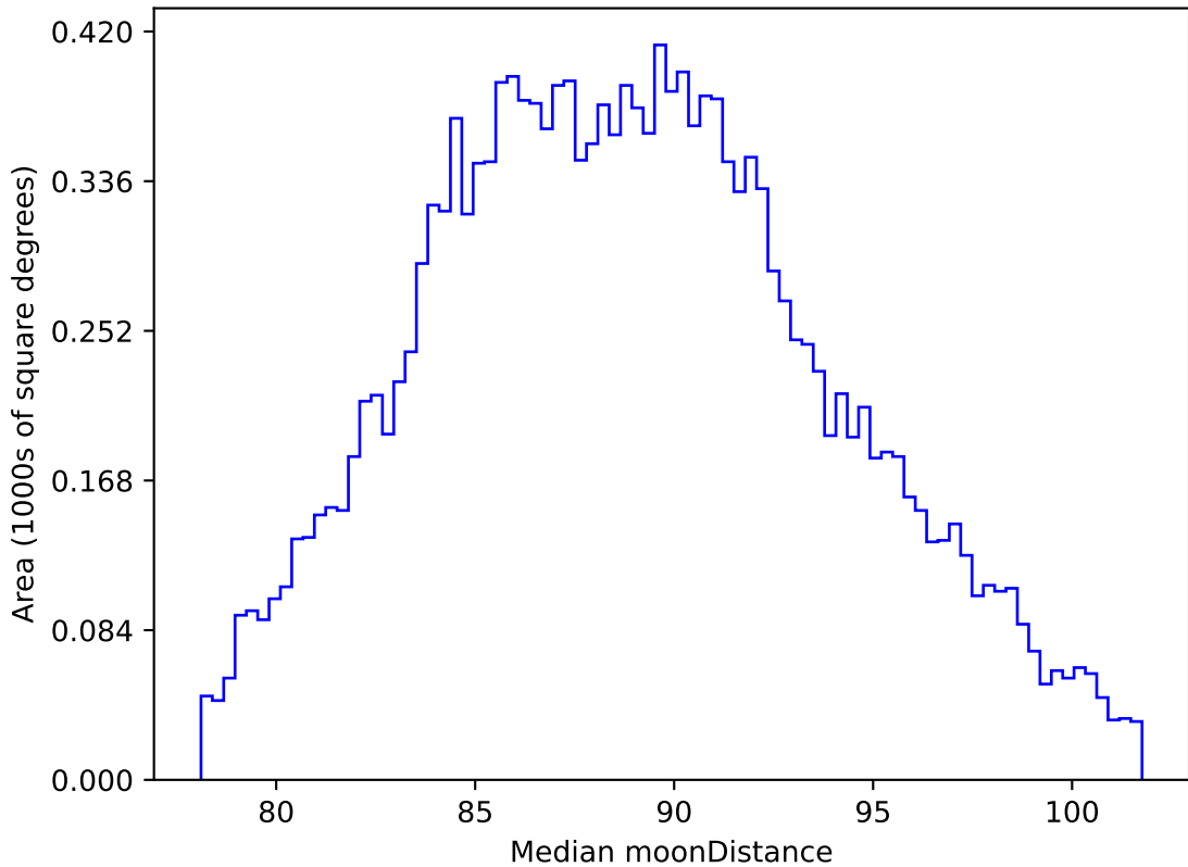
too_elab_r8_d3_giz_v3.4_10yrs WFD all bands: Median moonDistance
