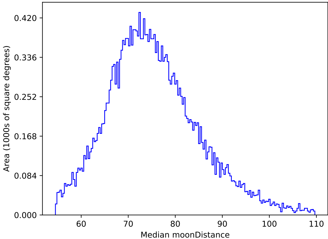
too_elab_r8_d3_giz_v3.4_10yrs All sky z band: Median moonDistance
