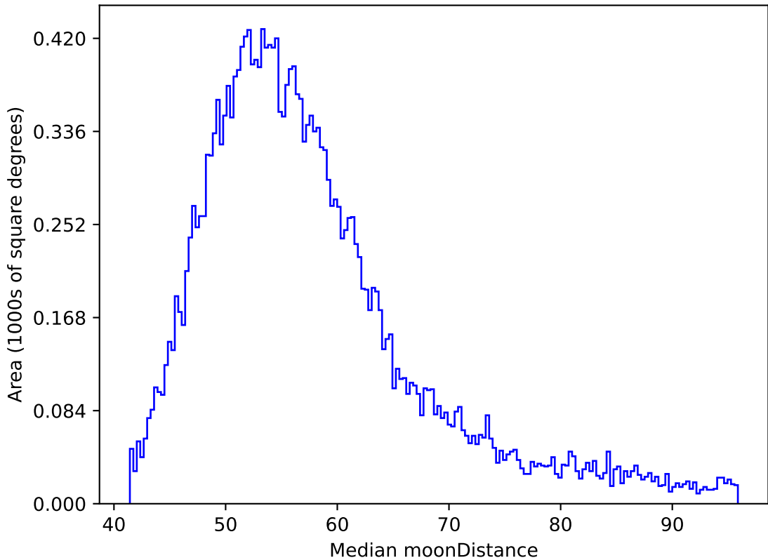
too_elab_r8_d3_giz_v3.4_10yrs All sky y band: Median moonDistance
