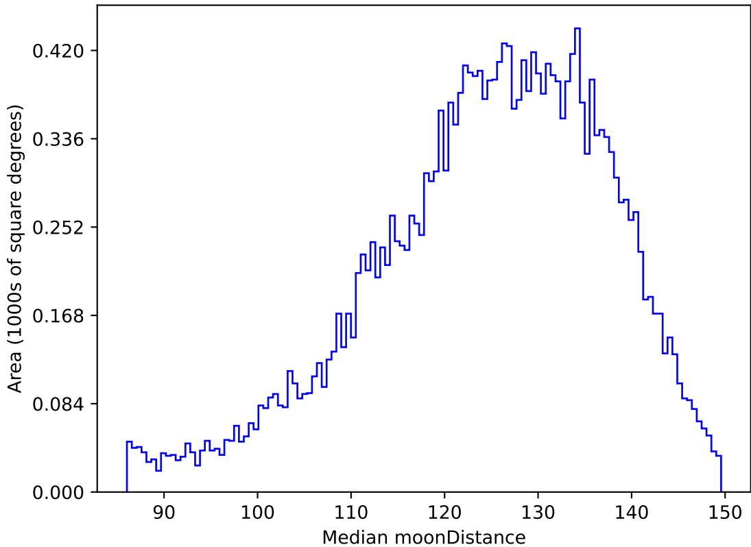
too_elab_r8_d3_giz_v3.4_10yrs All sky u band: Median moonDistance
