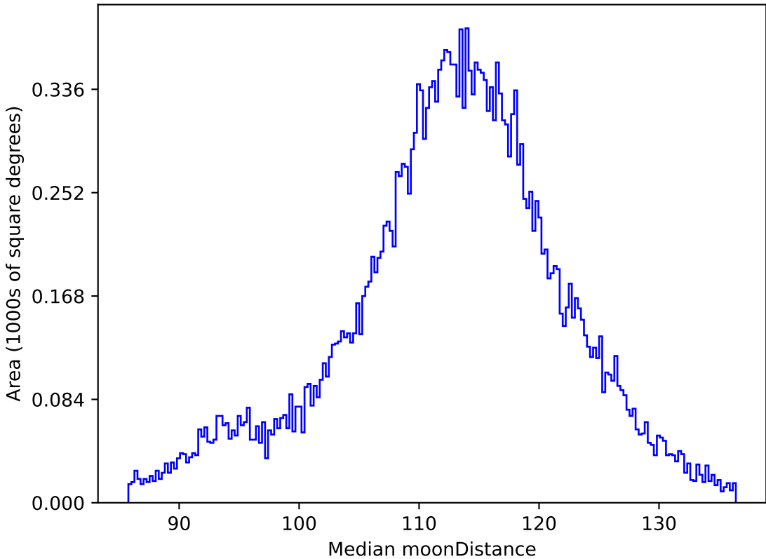
too_elab_r8_d3_giz_v3.4_10yrs All sky r band: Median moonDistance
