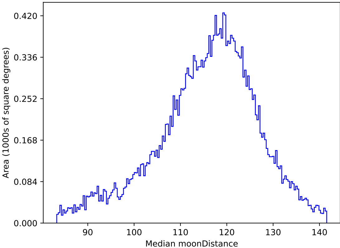
too_elab_r8_d3_giz_v3.4_10yrs All sky g band: Median moonDistance
