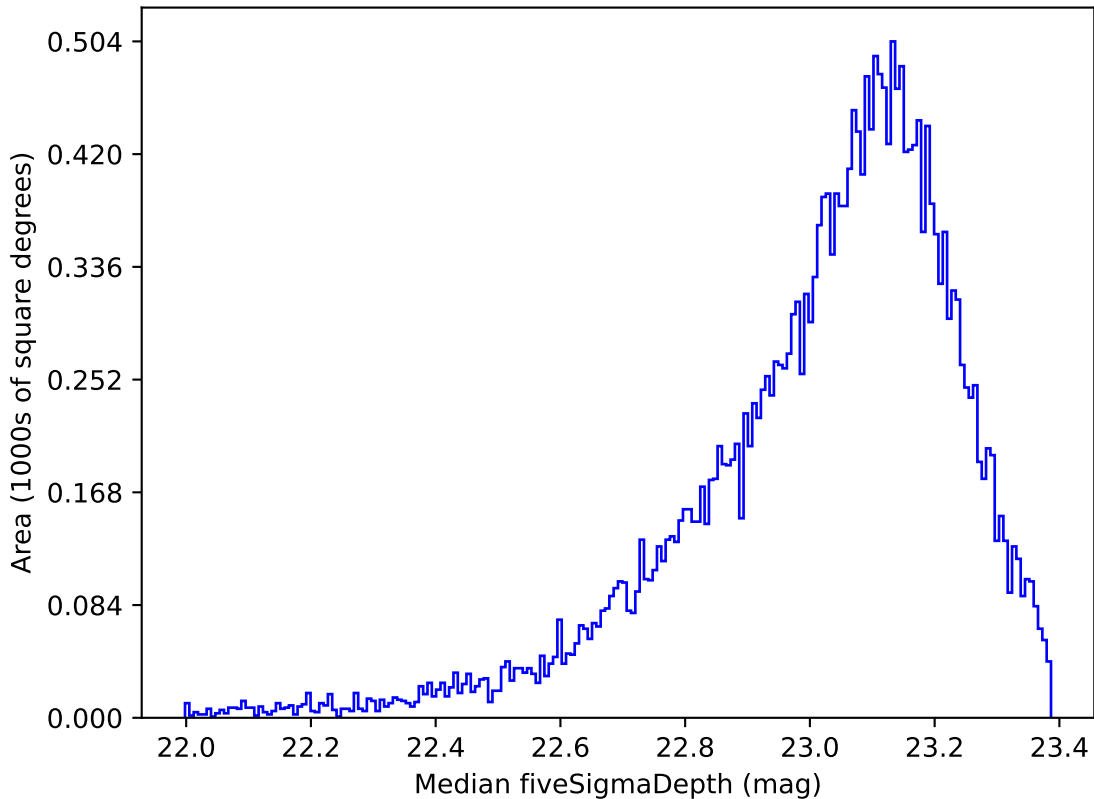
too_elab_r8_d3_giz_v3.4_10yrs Yr 1 z band: Median fiveSigmaDepth
