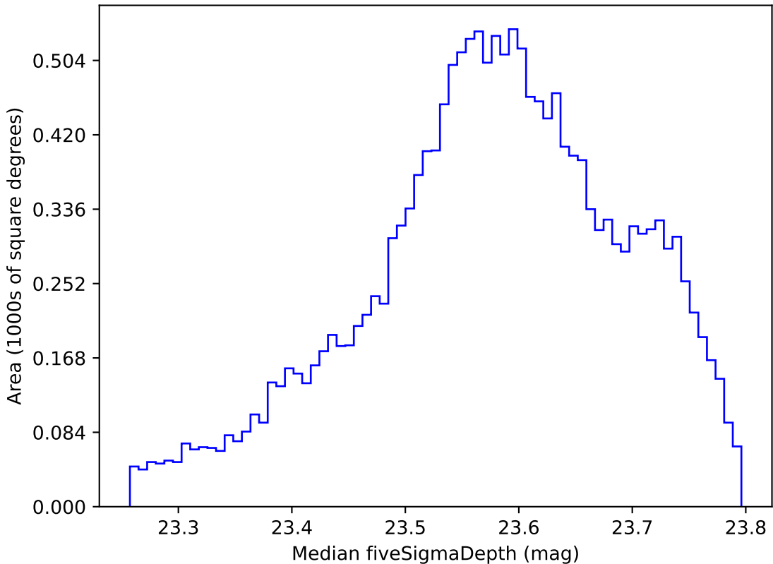
too_elab_r8_d3_giz_v3.4_10yrs WFD i band: Median fiveSigmaDepth
