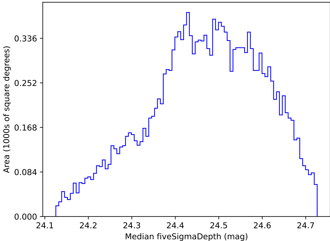
too_elab_r8_d3_giz_v3.4_10yrs WFD g band: Median fiveSigmaDepth
