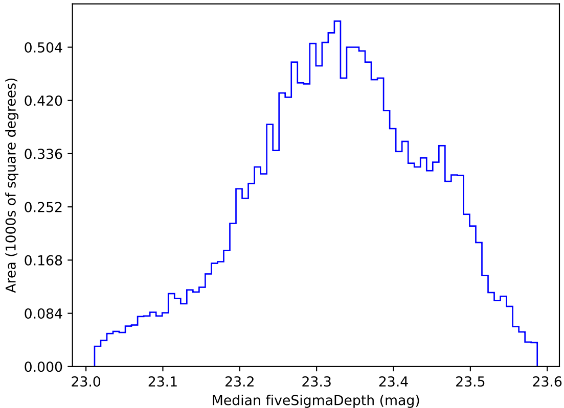
too_elab_r8_d3_giz_v3.4_10yrs WFD all bands: Median fiveSigmaDepth
