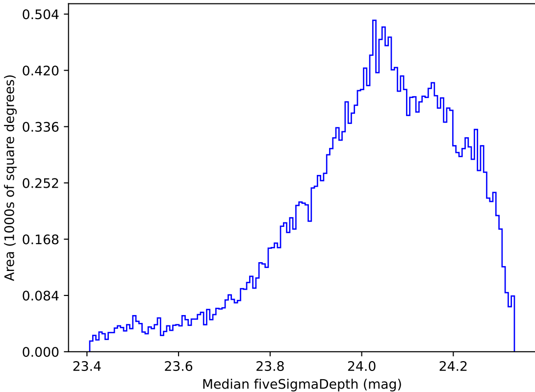
too_elab_r8_d3_giz_v3.4_10yrs All sky r band: Median fiveSigmaDepth
