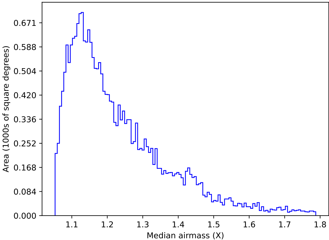
too_elab_r8_d3_giz_v3.4_10yrs Yr 1 u band: Median airmass
