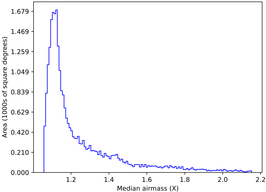
too_elab_r8_d3_giz_v3.4_10yrs Yr 1 r band: Median airmass
