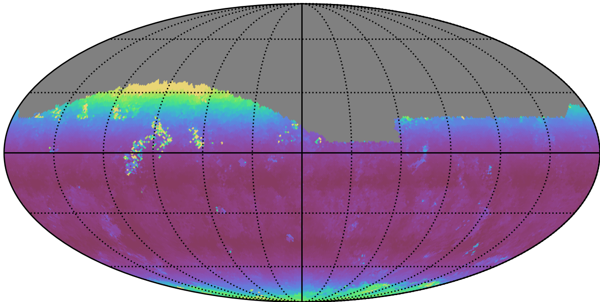
too_elab_r8_d3_giz_v3.4_10yrs Yr 1 i band: Median airmass
