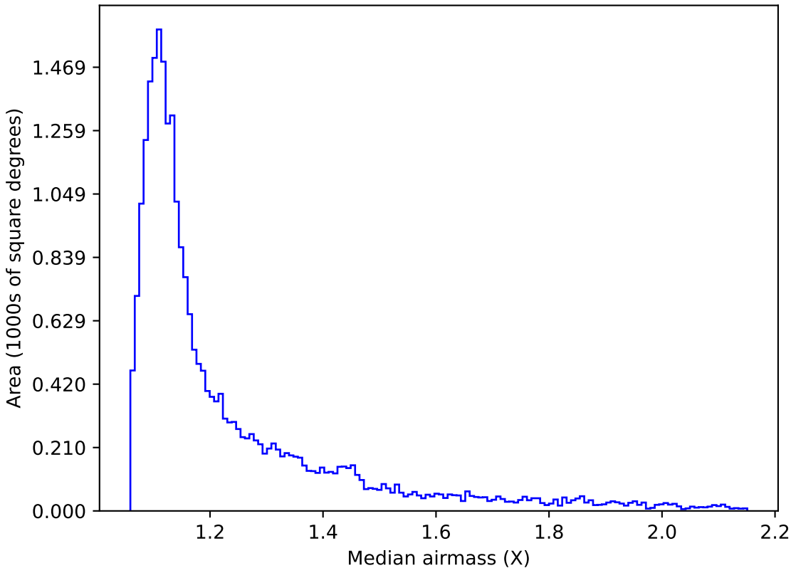
too_elab_r8_d3_giz_v3.4_10yrs Yr 1 i band: Median airmass
