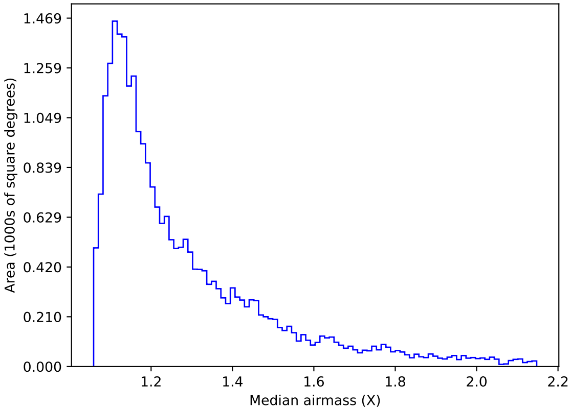
too_elab_r8_d3_giz_v3.4_10yrs Yr 1 g band: Median airmass
