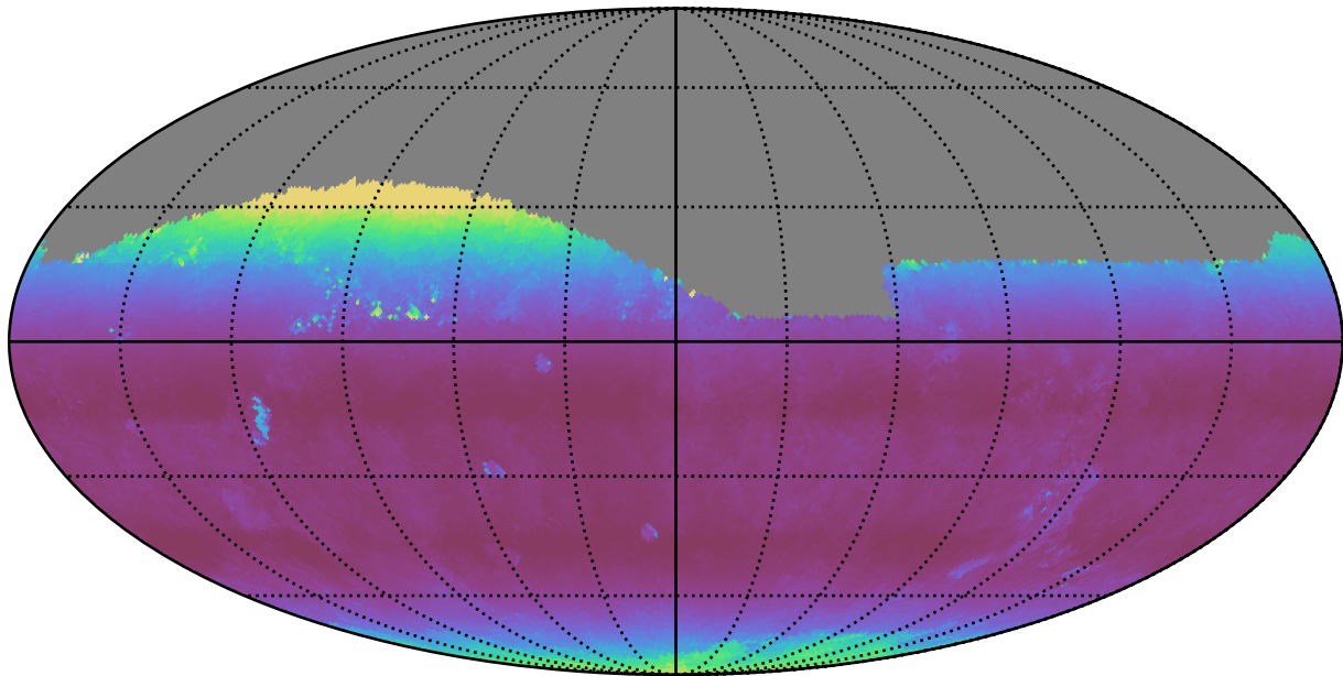
too_elab_r8_d3_giz_v3.4_10yrs Yr 1 all bands: Median airmass
