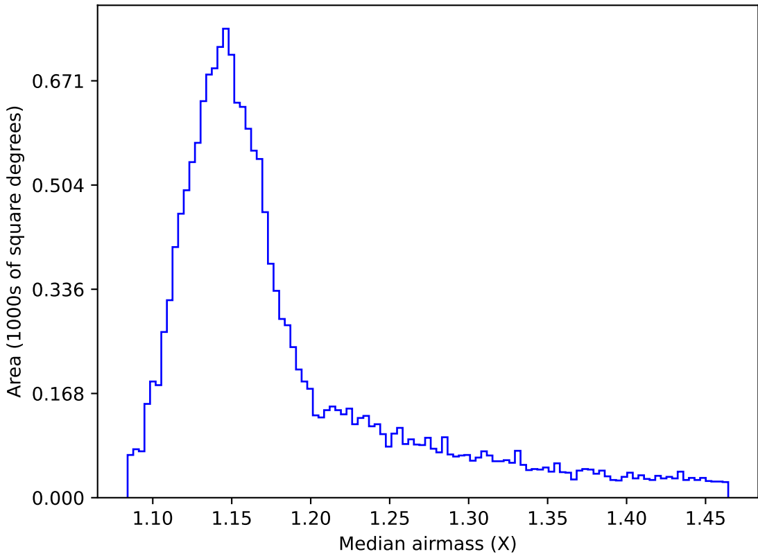
too_elab_r8_d3_giz_v3.4_10yrs WFD z band: Median airmass
