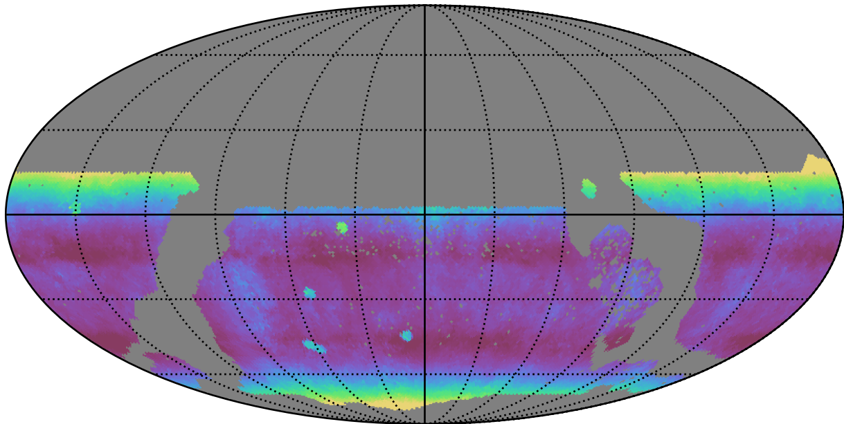
too_elab_r8_d3_giz_v3.4_10yrs WFD y band: Median airmass
