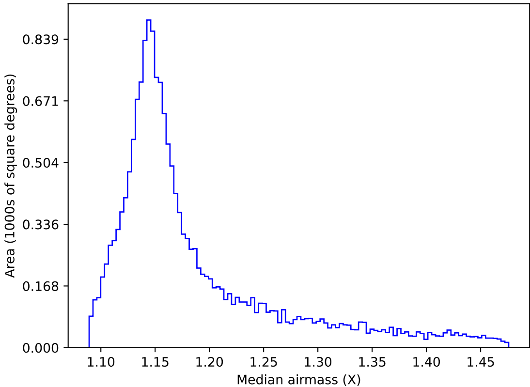
too_elab_r8_d3_giz_v3.4_10yrs WFD y band: Median airmass
