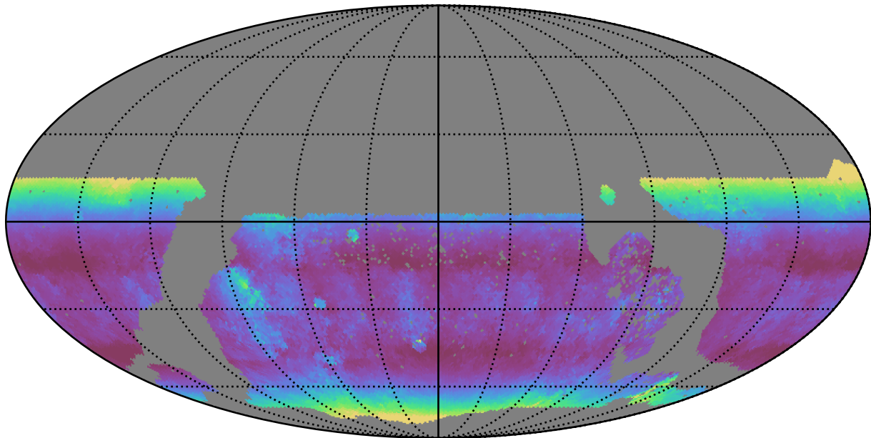
too_elab_r8_d3_giz_v3.4_10yrs WFD u band: Median airmass
