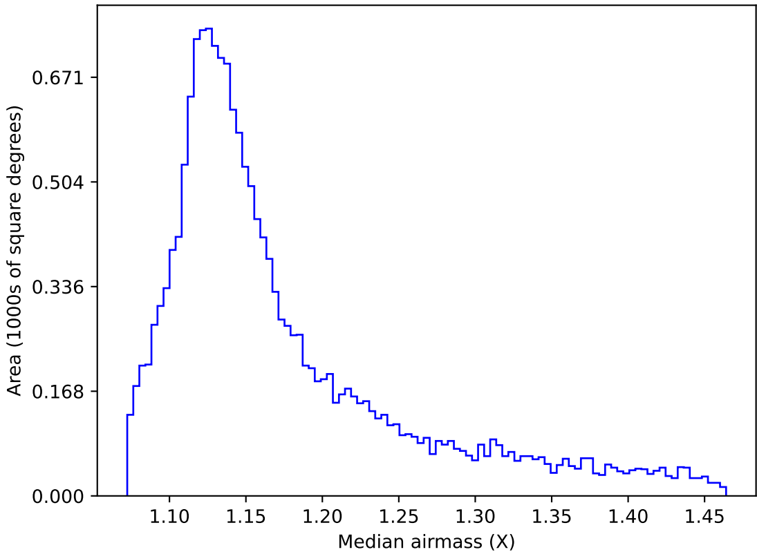
too_elab_r8_d3_giz_v3.4_10yrs WFD u band: Median airmass
