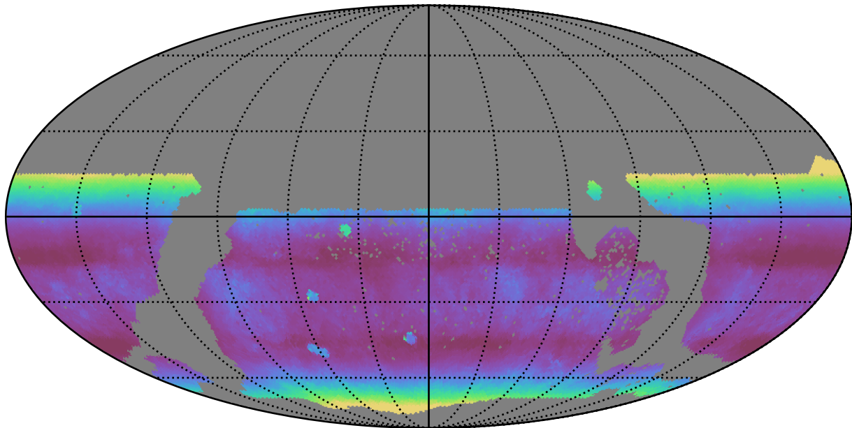
too_elab_r8_d3_giz_v3.4_10yrs WFD r band: Median airmass
