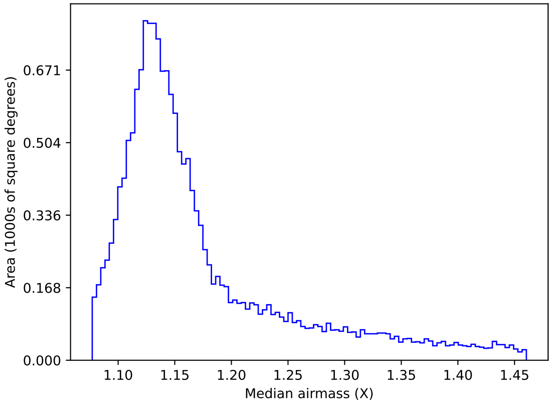
too_elab_r8_d3_giz_v3.4_10yrs WFD r band: Median airmass
